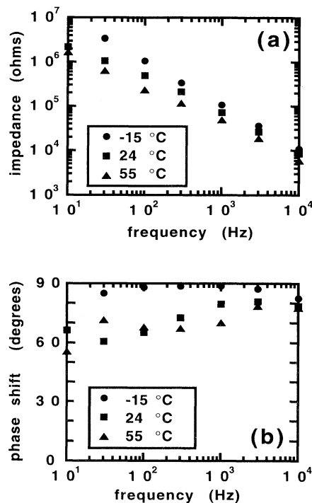
FIG. 12. Magnitude (a) and phase (b) of the complex impedance of the PDLC film as a function of frequency are shown for several sample temperatures.
